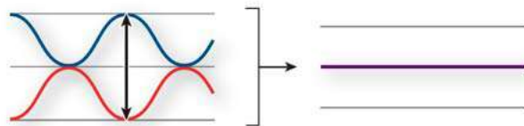
Out-of-phase waves cancel each other out.
